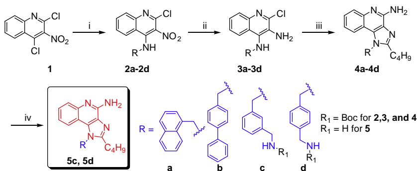
Scheme 1. Syntheses of N^1 -substituted imidazoquinolines. Reagents: (i) RNH_2 , Et_3N , CH_2Cl_2 ; (ii) Pt/C , H_2 , Na_2SO_4 , EtOAc ; (iii) (a) C_4H_9COCl , Et_3N , THF ; (b) NH_3/MeOH , 150\text{ }^\circ C ; (iv) HCl/dioxane .
